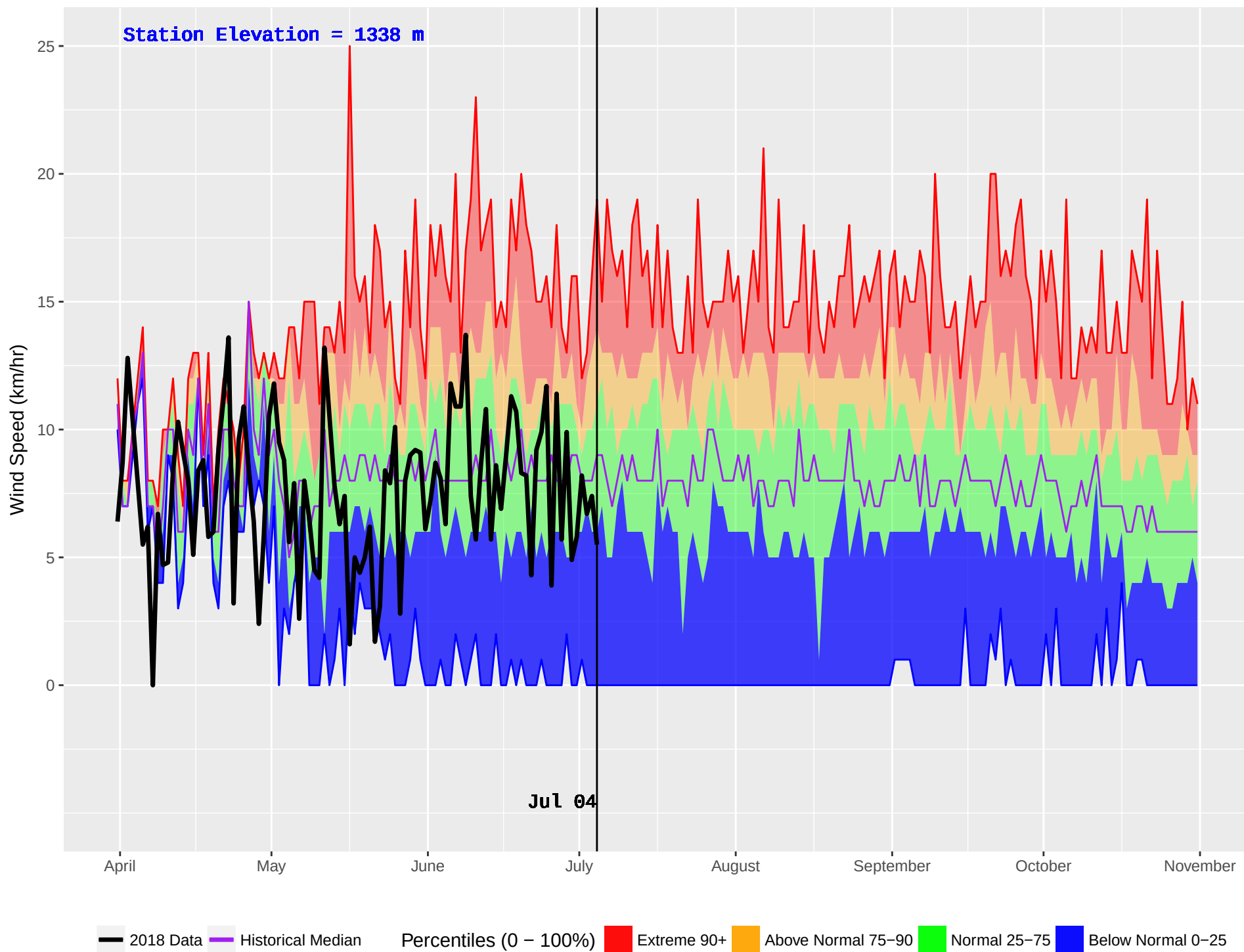
EIGHT MILE (391) : Historical (1980–2016) and Current (2018) Noon Wind Speed
