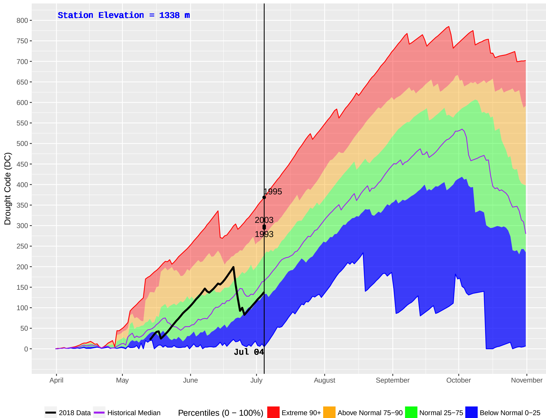
EIGHT MILE (391) : Historical (1980–2016) and Current (2018) Noon Drought Code (DC)
